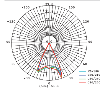
Curva fotometrica / Distribution curve
