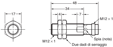
E2A-M12KS04-M1-□□/E2A-S12KS04-M1-□
