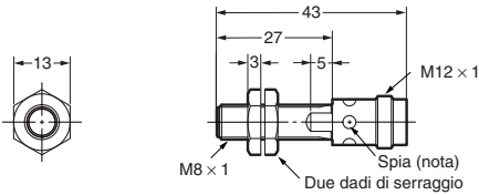
E2A-S08KS02-M1-□□
