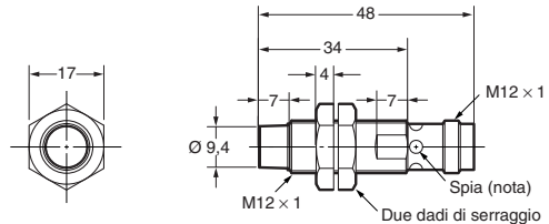
E2A-M12KN08-M1-□□/E2A-S12KN08-M1-□
